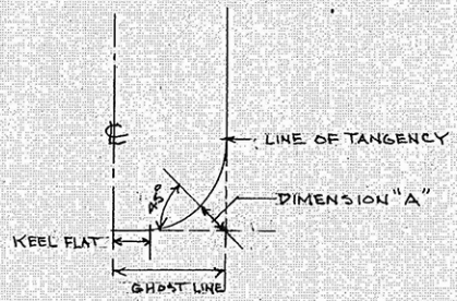
TYPICAL SEC. THRU BALLAST SHOWING MEASUREMENT POINTS, NOT TO SCALE
